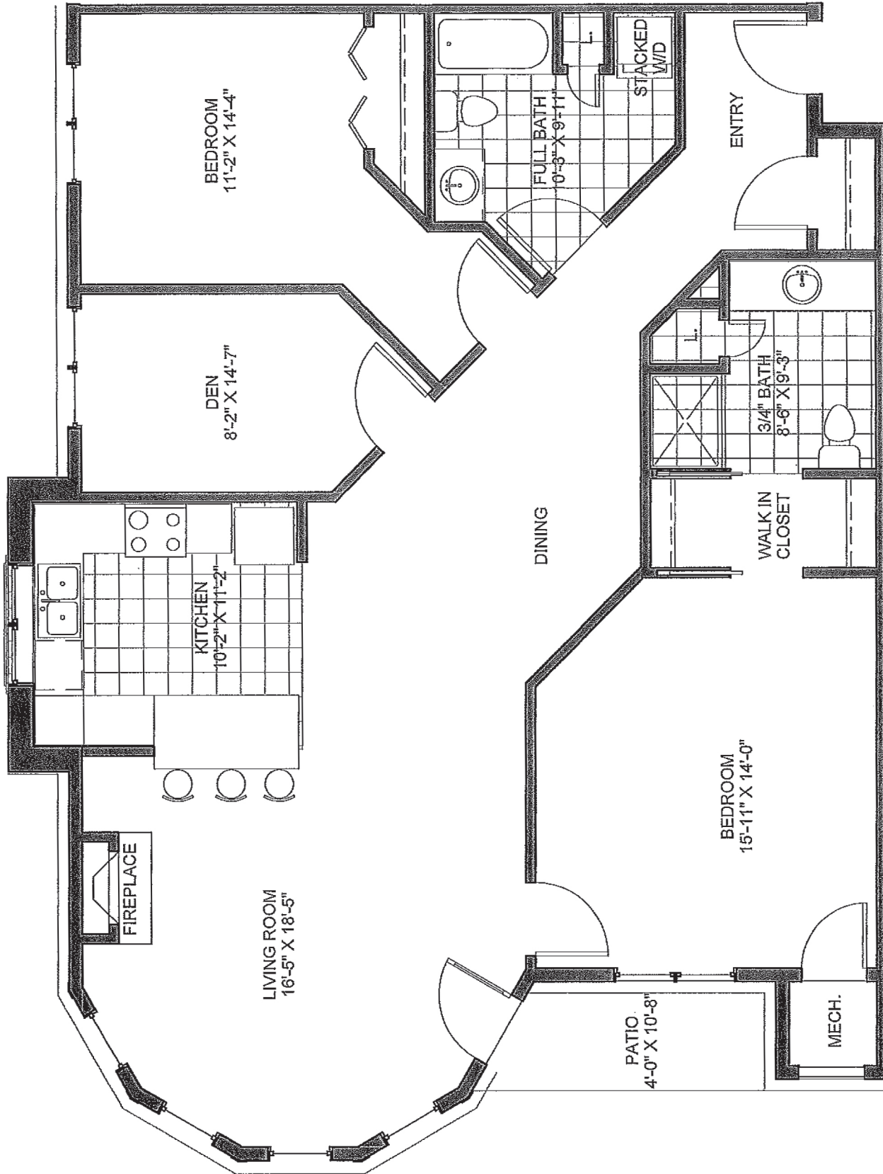
THE PINEHURST TWO BEDROOM + DEN 1,488 SQ. FT.
